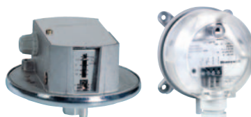
HCD, DPT, DPS Differential pressure switches and transmitters for gases, air and exhaust gases
